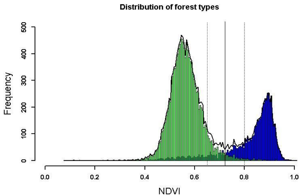
Figure 3. Distribution of broadleaved (green) and coniferous (blue) tree species in the reference data extracted from the Landsat 8 image. The black line depicts the sum of both classes. The vertical black line indicates the minimum turning point, the vertical dotted lines the distance of one-half standard deviation in the dataset, which is used as range for threshold parameterization.
